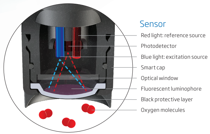
HI764113-1 Smart Cap
